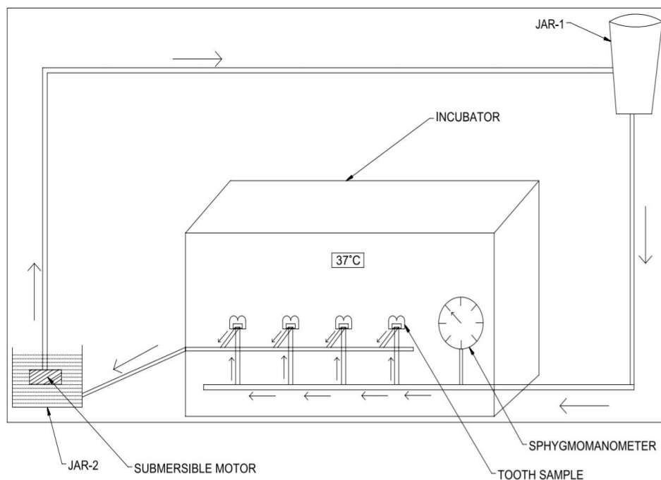
Figure 1: Intra pulpal pressure simulation model with tooth mounted on circular disc and temperature maintained at 37°C
