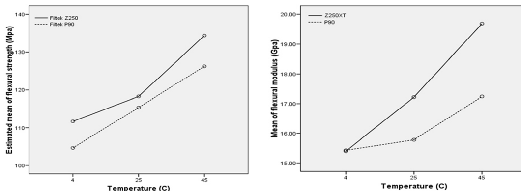
Figure 2: Mean of flexural strength and modulus of the resin composites
